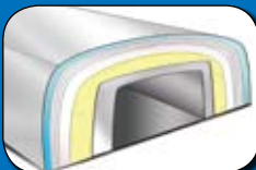
8-10mm Thick, Oven Cured 6 Layer "Tough Bond" Shell
